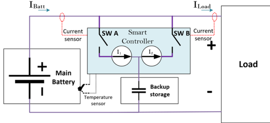
Figure 2.2: Schematic diagram of the test circuit
